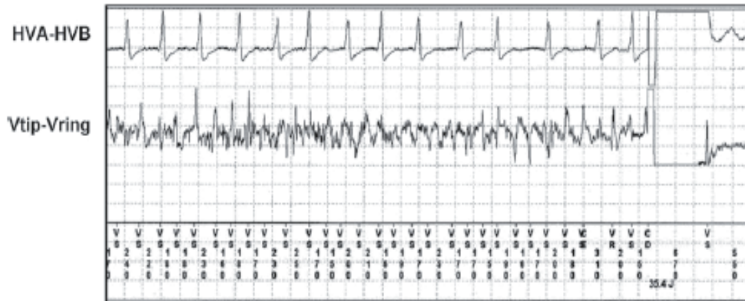
Figure 1. Stored electrogram
