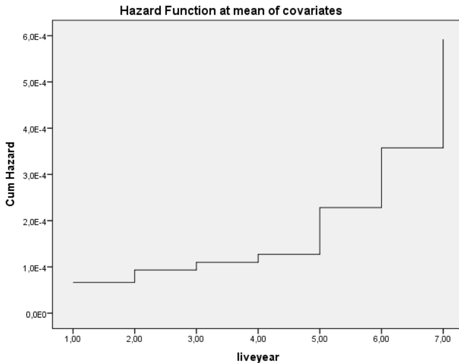
Figure 2. Hazard function analysis
