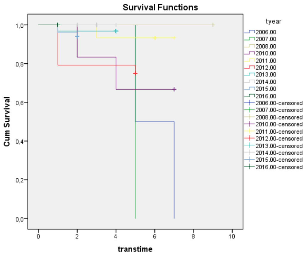
Figure 1. Survival functions
